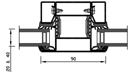
Montant - traverse Mullion - transom Pfosten - Riegel
